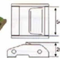
CB01-72 2" Cambuckle, 50mm B.S.: 700Kgs/ 1540Lbs
