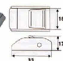
CB06-1518 3/4" Cambuckle, 18mm B.S. : 150Kgs/ 300Lbs
