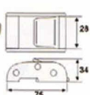
CB08-81 1" Cambuckle, w/floating Cam, 25mm, B.S. : 800Kgs/ 1760Lbs
