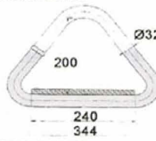
LDR109-32240
