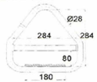
LDR108-28284
