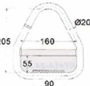
LDR105-20160
