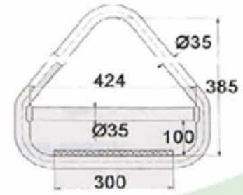
LDR110-35424
