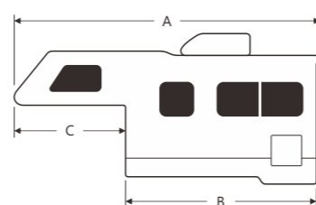
A: Overall length B: Floor length C: Cabover length
